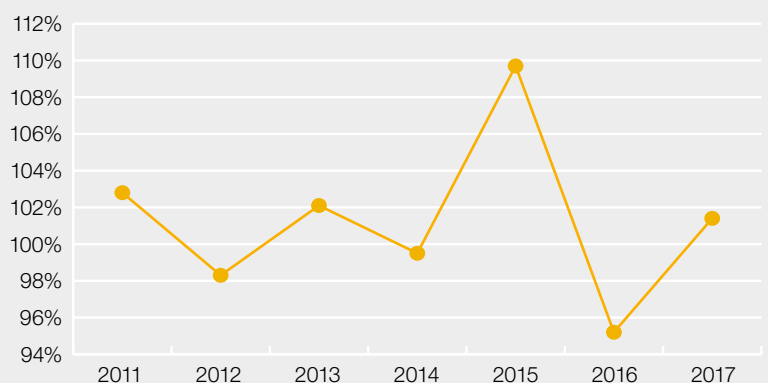
Figure 13: Annual energy deviation due to wind speed – 2011 to 2017
